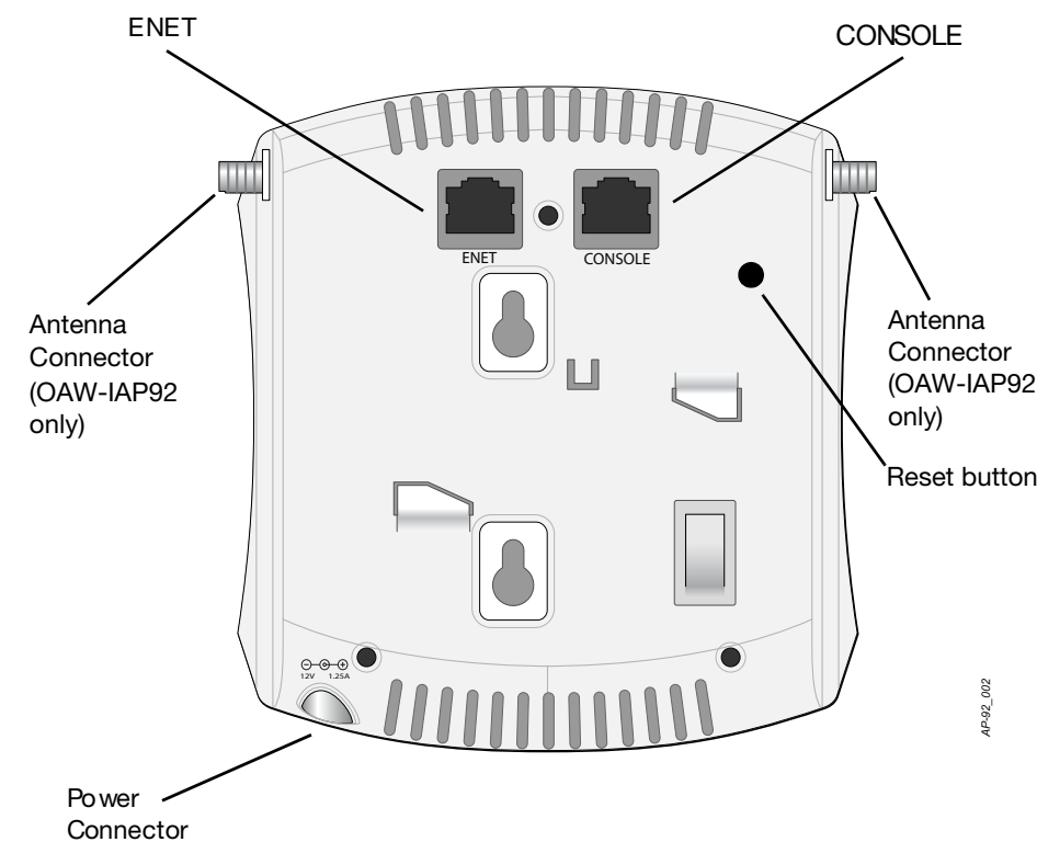
Figure 3 Rear (OAW-IAP92 Shown)
