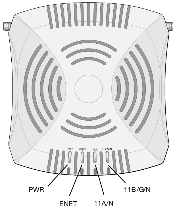
Figure 2 Front (OAW-IAP92 Shown)
