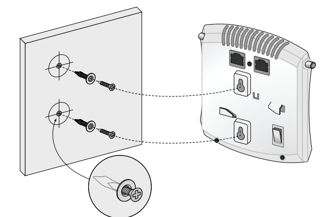
Figure 4 Installing the OAW-IAP92/OAW-IAP93 Access Point on a Wall
